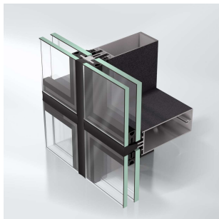
Structurally glazed with sealant
